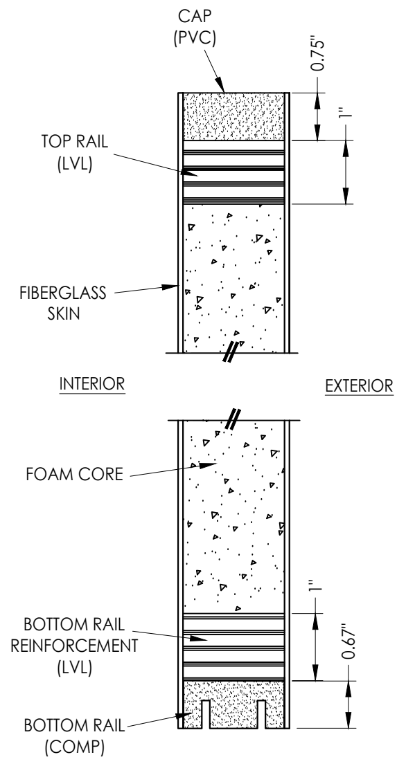
2 VERTICAL CROSS SECTION
