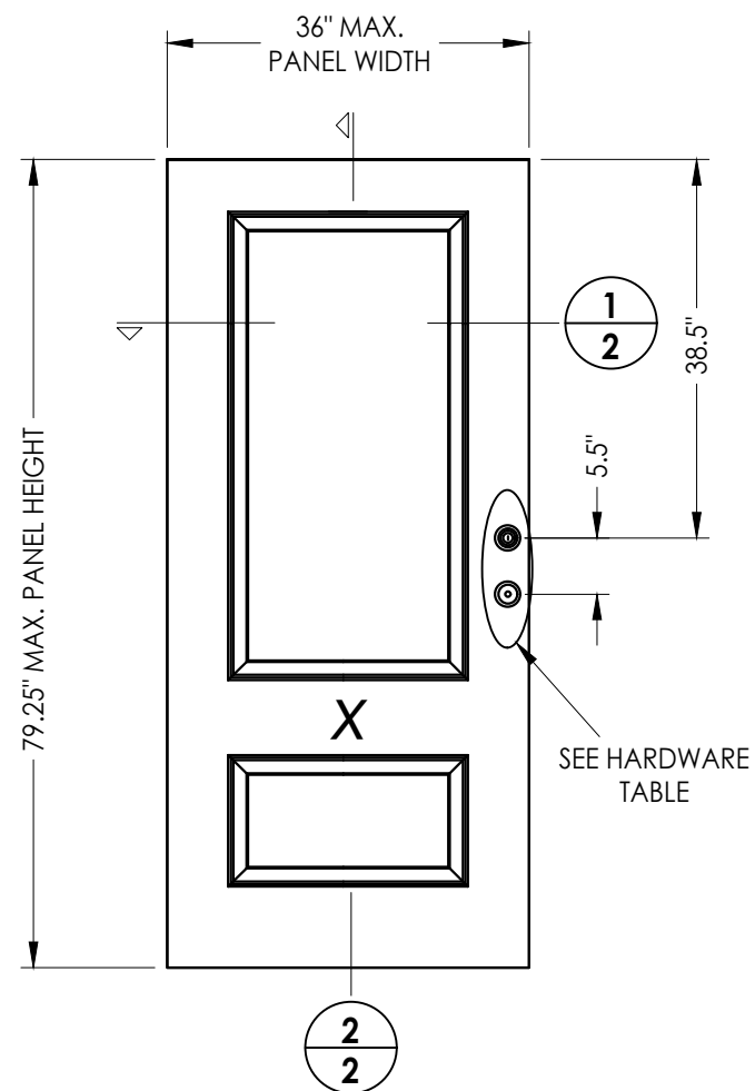
40 FIBERGLASS DOOR PANEL
